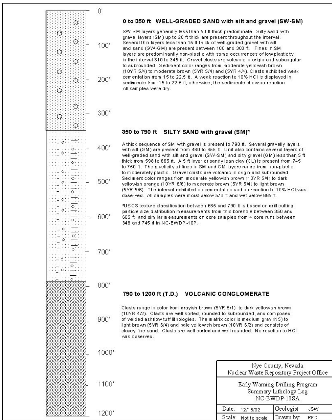
Figure H1 Summary Lithologic Log for Well NC-EWDP-10SA
