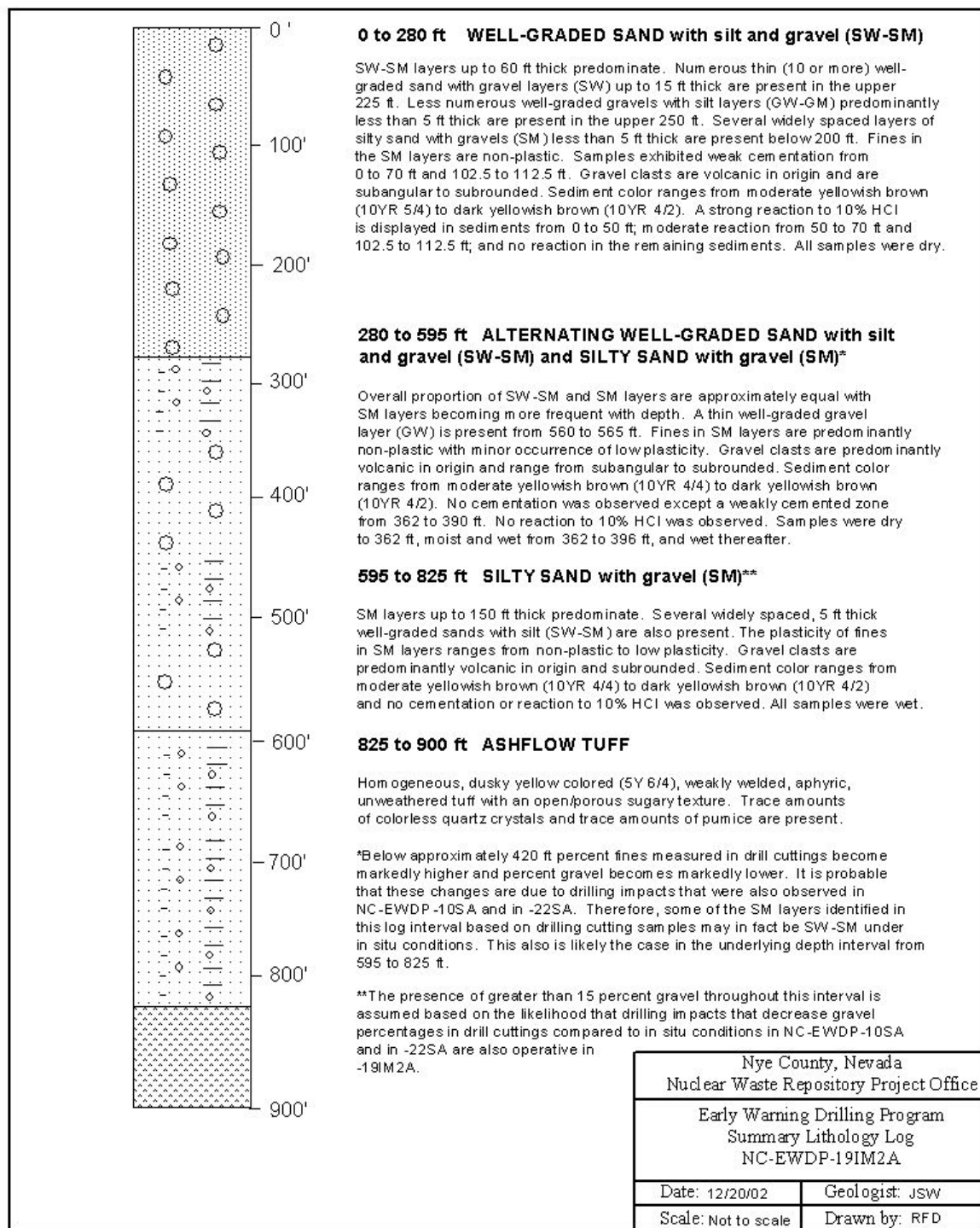
Figure H2 Summary Lithologic Log for Well NC-EWDP-19IM2A
