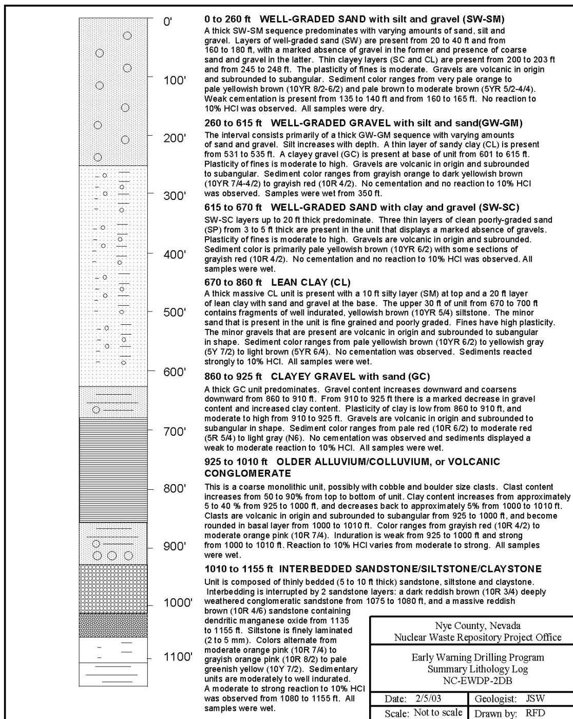
Figure H6 Summary Lithologic Log for Well NC-EWDP-2DB
