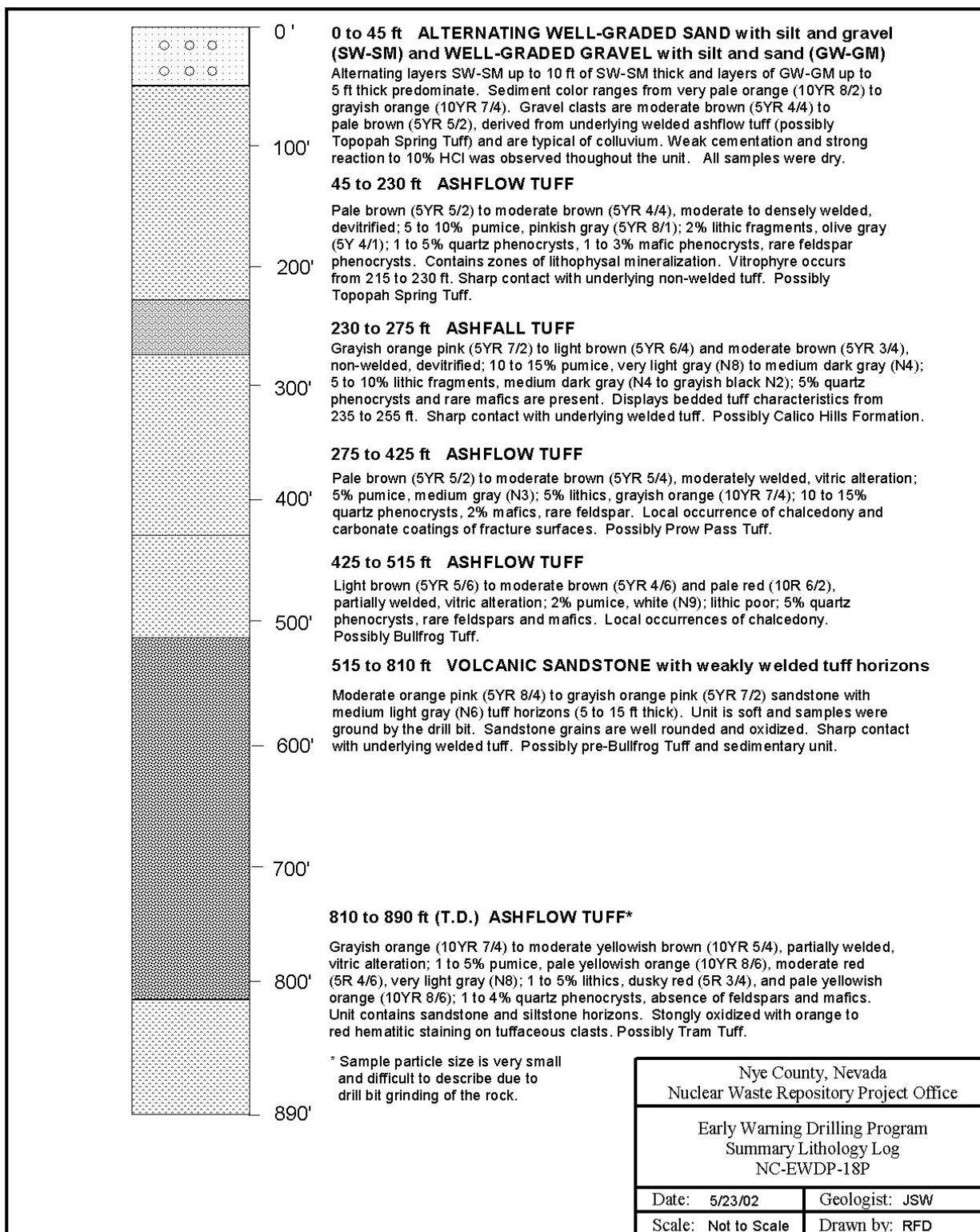
Figure H4 Summary Lithologic Log for Well NC-EWDP-18P
