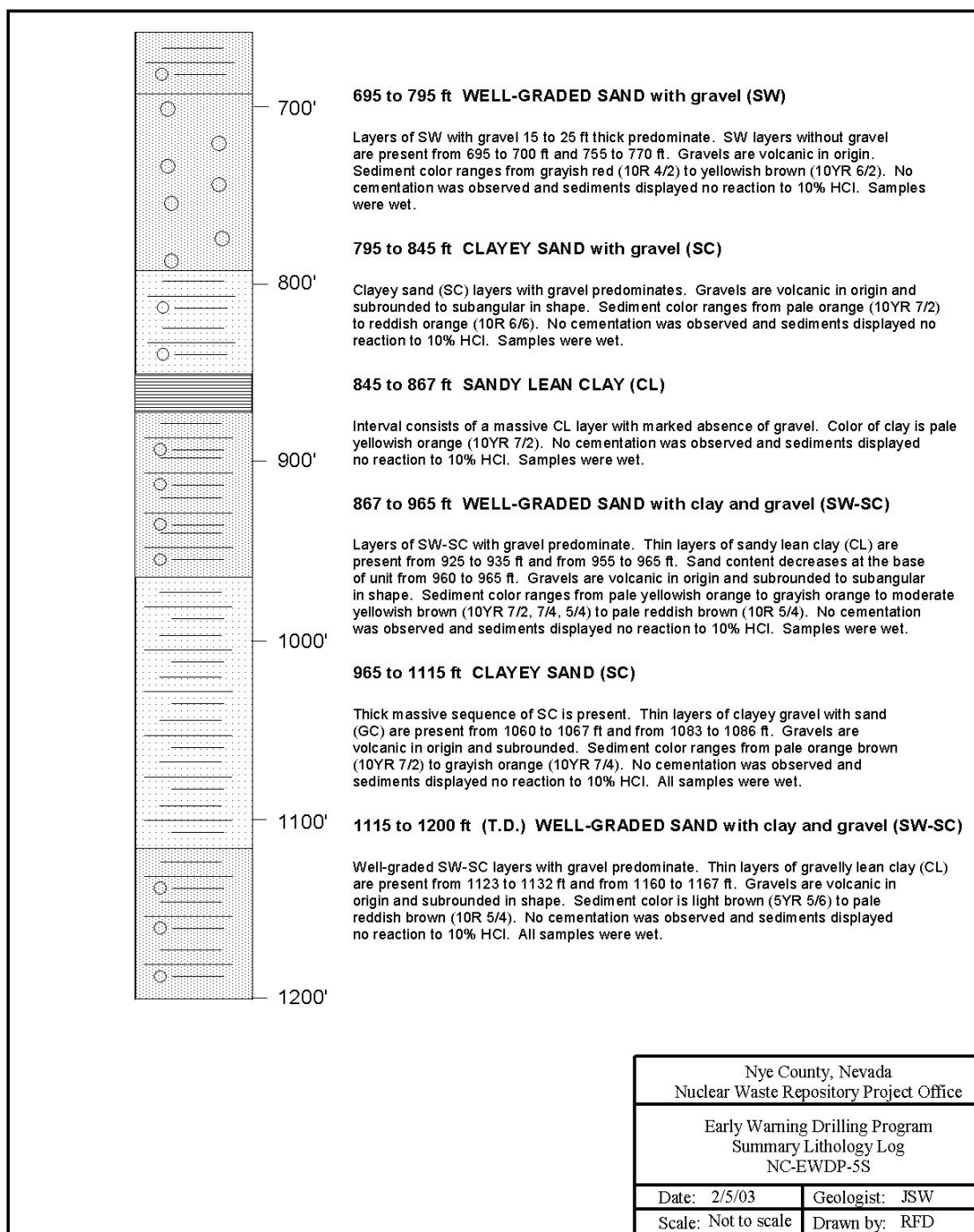
Figure H8 Summary Lithologic Log for Well NC-EWDP-5S (695 to 1,200 ft)
