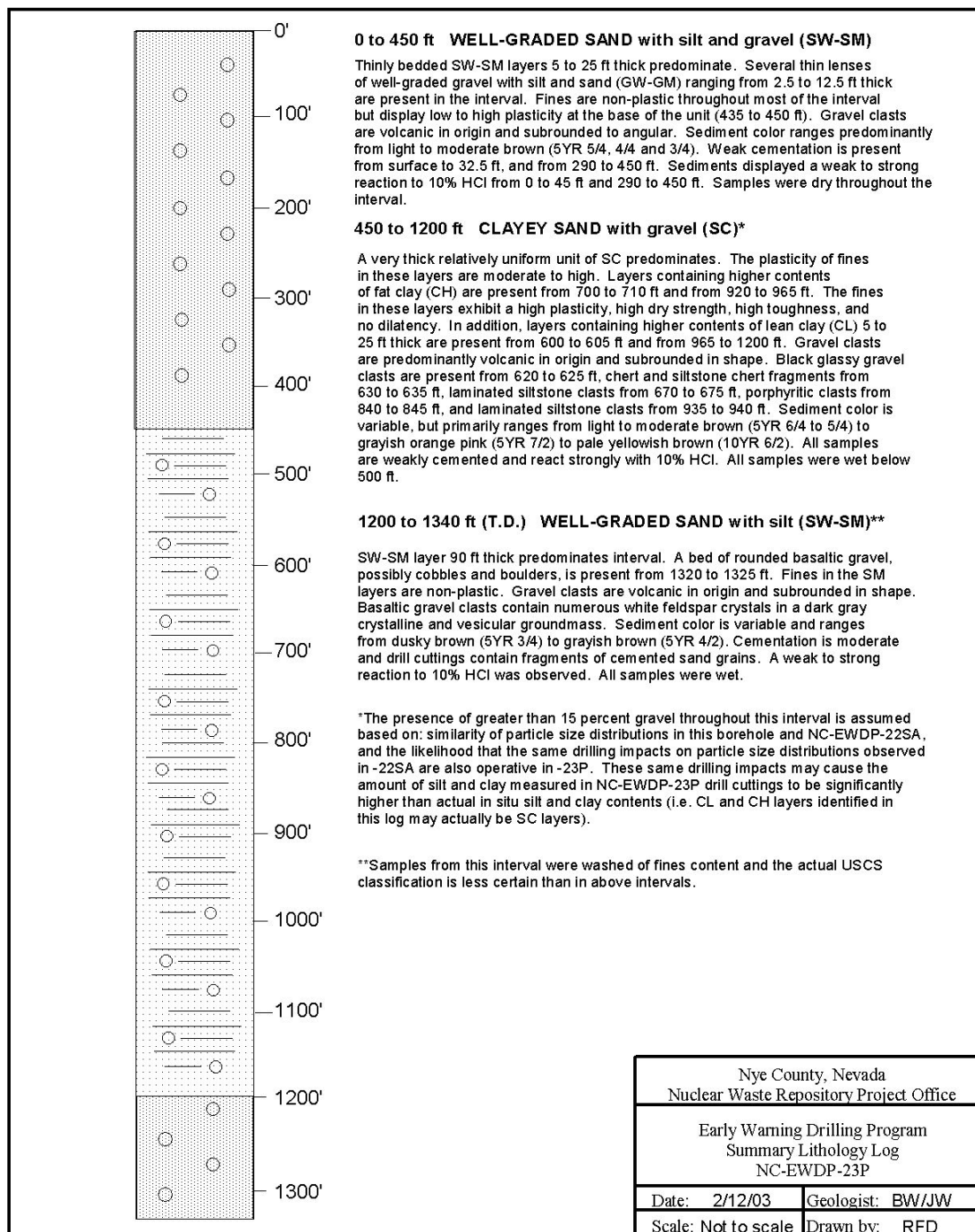
Figure H5 Summary Lithologic Log for Well NC-EWDP-23P
