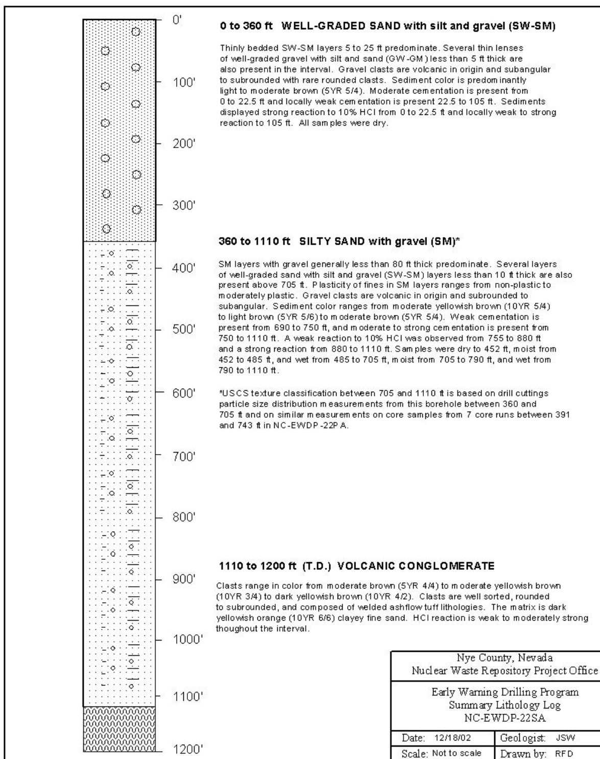
Figure H3 Summary Lithologic Log for Well NC-EWDP-22SA
