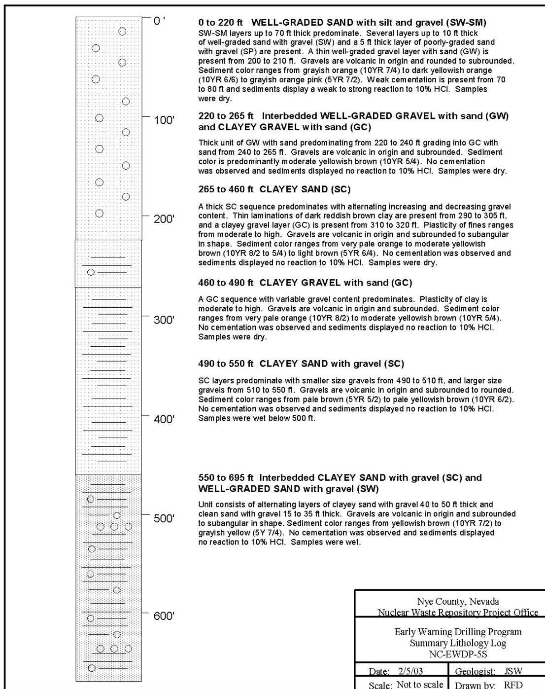
Figure H7 Summary Lithologic Log for Well NC-EWDP-5S (0 to 695 ft)
