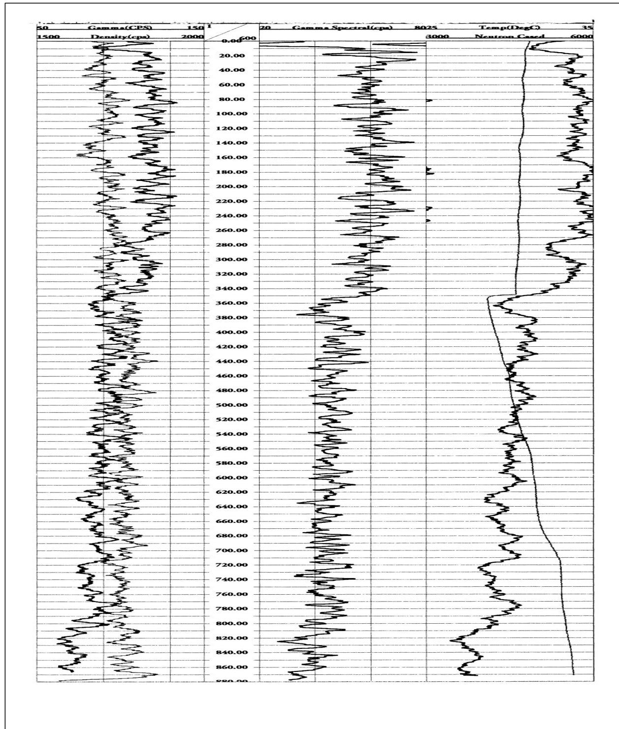
Figure G2 Drill-String Geophysical Logs for Well NC-EWDP-19IM1A
