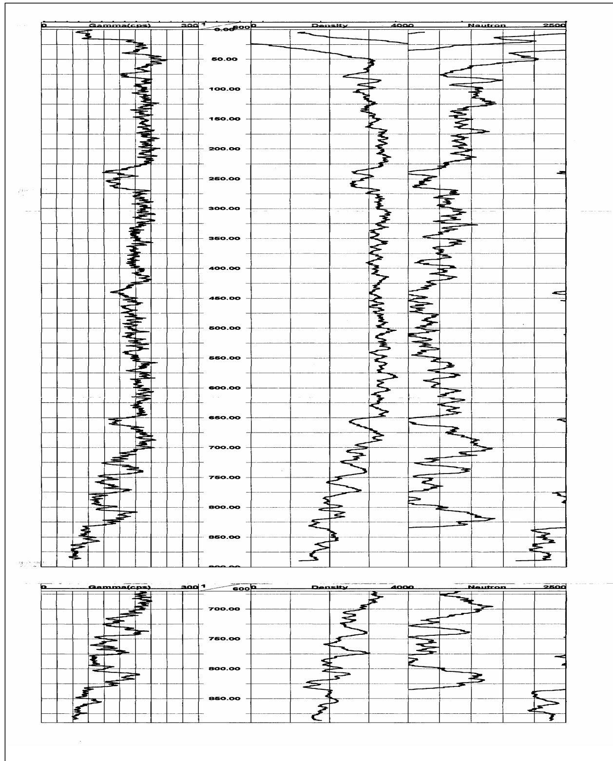
Figure G9 Well-Completion Geophysical Logs for Well NC-EWDP-18P
