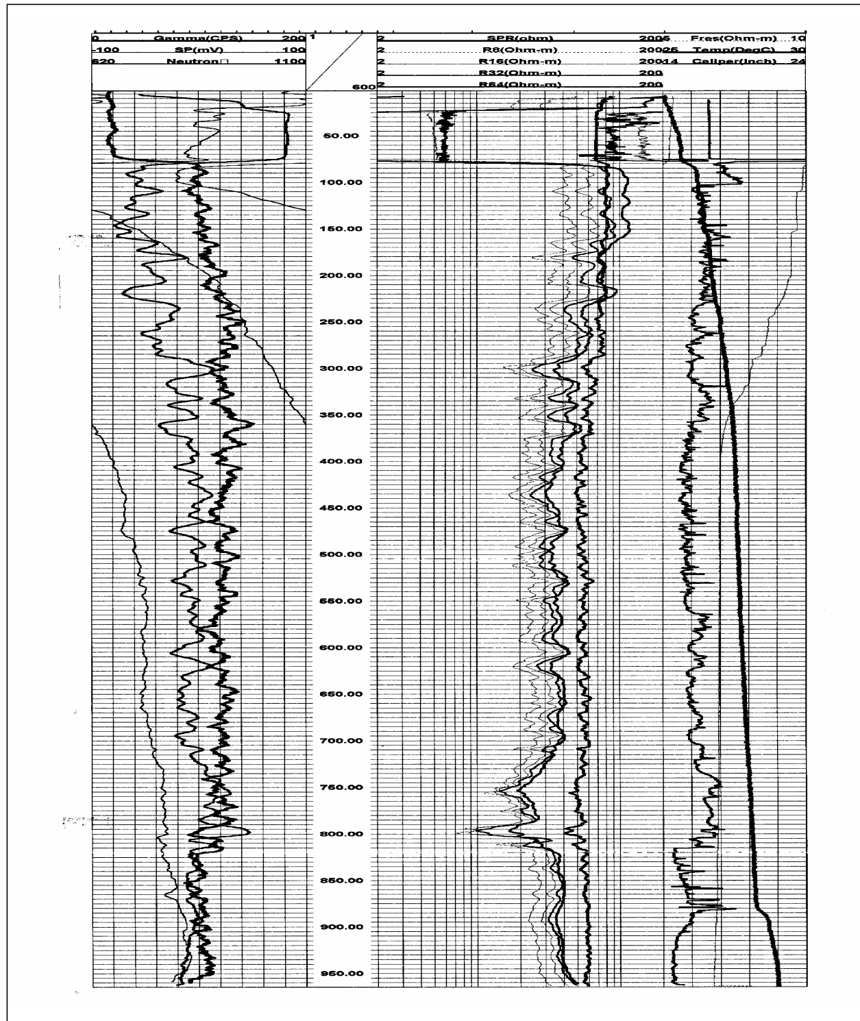
Figure G6 Open-Hole Geophysical Logs for Well NC-EWDP-19IM2
