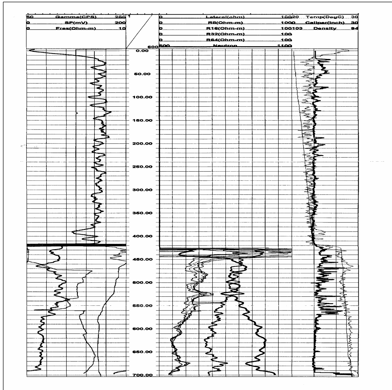
Figure G8 Open-Hole Geophysical Logs for Well NC-EWDP-23P
