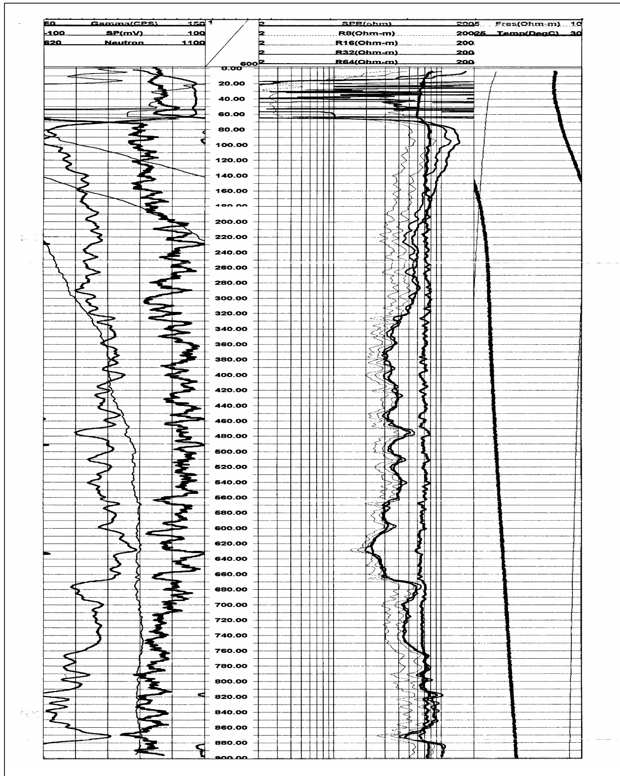
Figure G5 Open-Hole Geophysical Logs for Well NC-EWDP-10S
