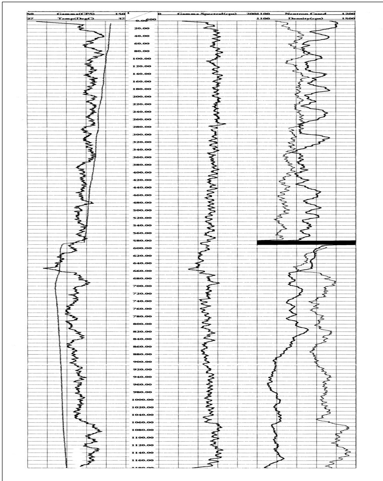
Figure G1 Drill-String Geophysical Logs for Well NC-EWDP-10SA
