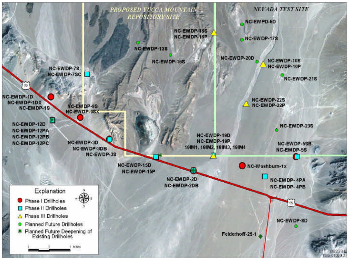
Figure 4.1-1 Location of Early Warning Drilling Program Drillholes
