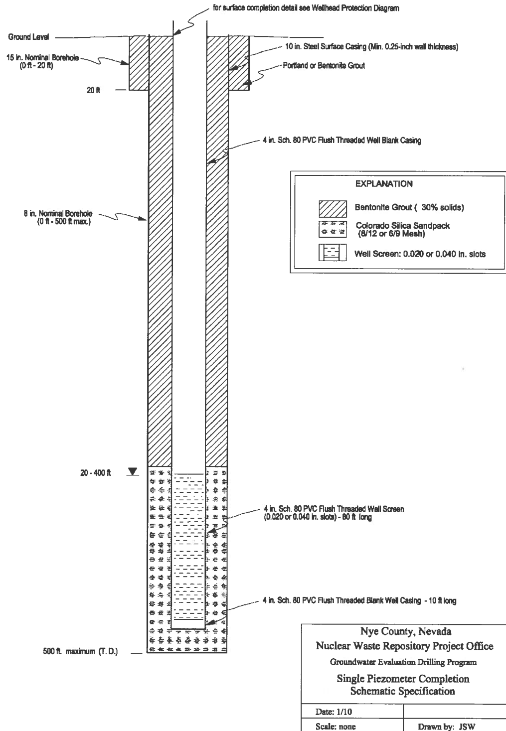
Attachment A Figure 2 Schematic Well Completion Diagram for GWE Piezometer Wells
