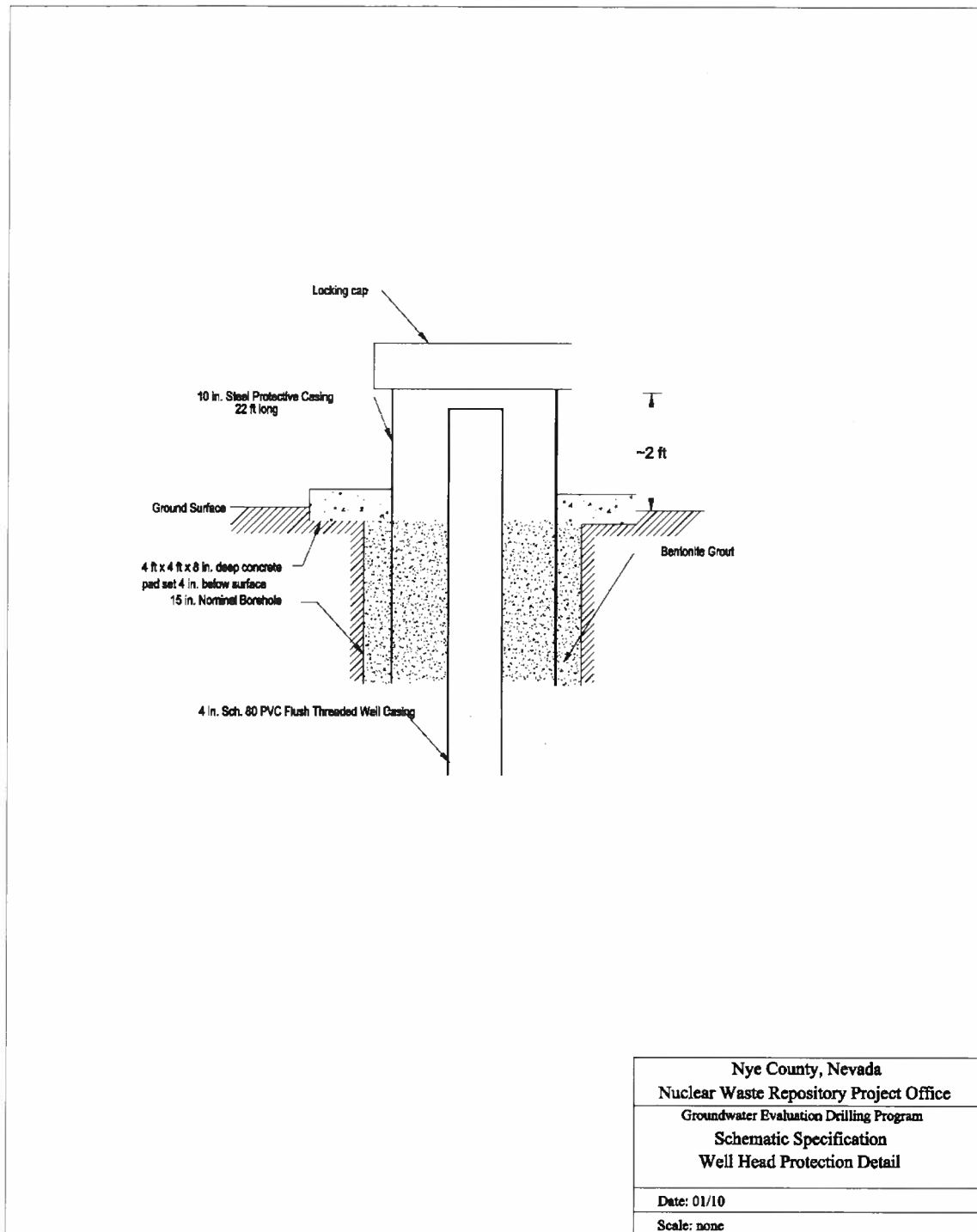
Attachment A Figure 3 Schematic Well Head Protection detail for GWE Piezometer Wells
