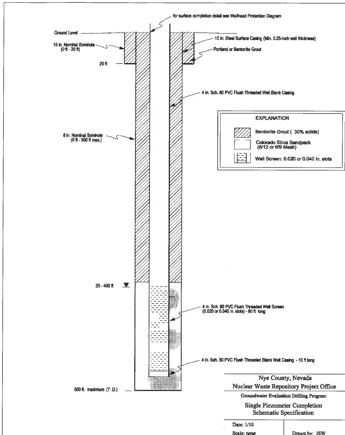
Figure 2 Typical Piezometer Subsurface Completion Diagram
